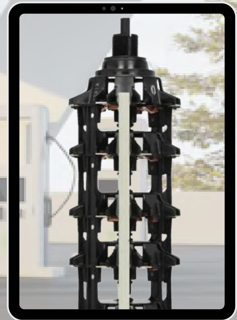
Bushing
